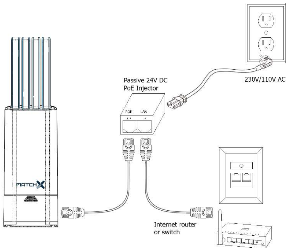
Figure 2.1: Connection of MX1901/2 Gateway.
